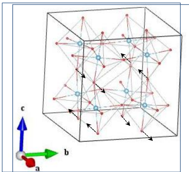
O2_B1g_2
