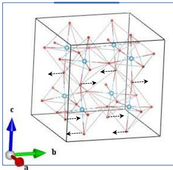
O2_B1g_1
