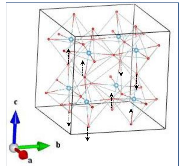
O2_B3g
