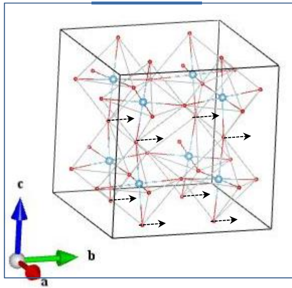
O2_B2u_1
