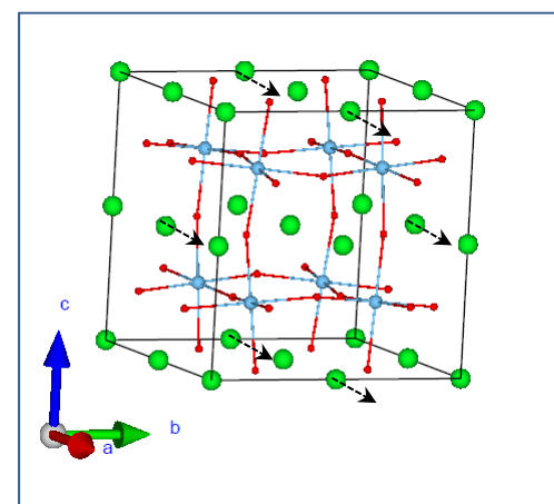
Sr_4_B3u
