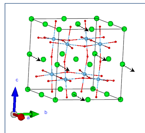
Sr_3_B3u
