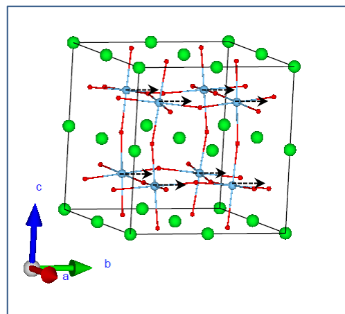
T_B2u_2
