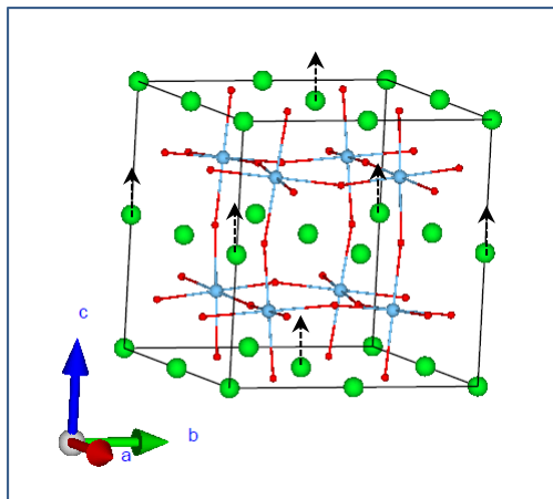
Sr_3_B1u
