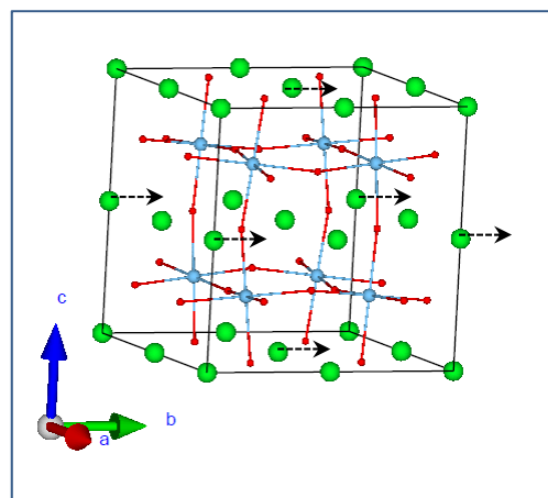
Sr_3_B2u
