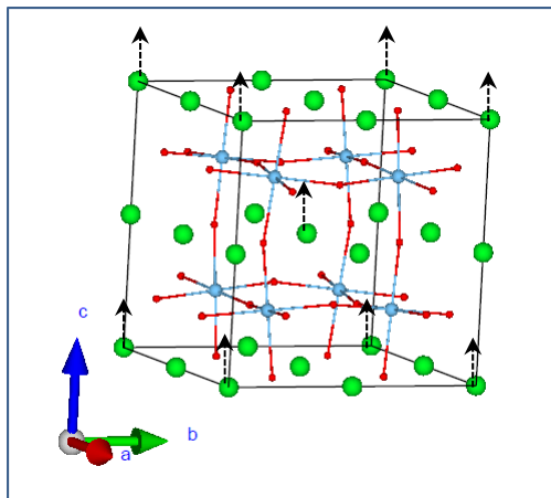
Sr_1_B1u
