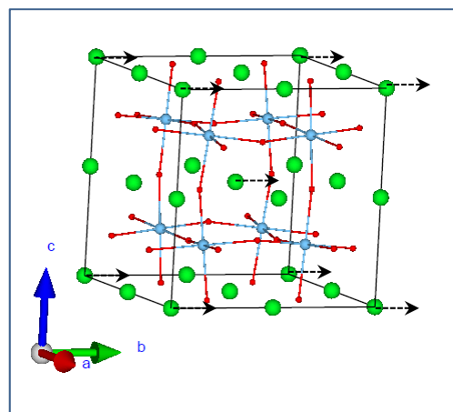
Sr_1_B2u
