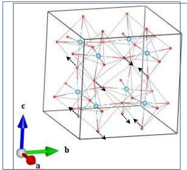
O2_B2u_2
