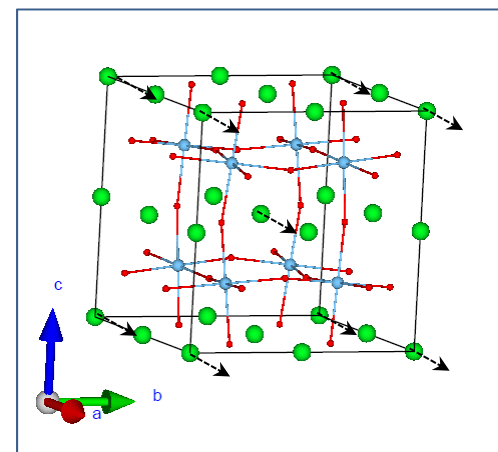
Sr_1_B3u
