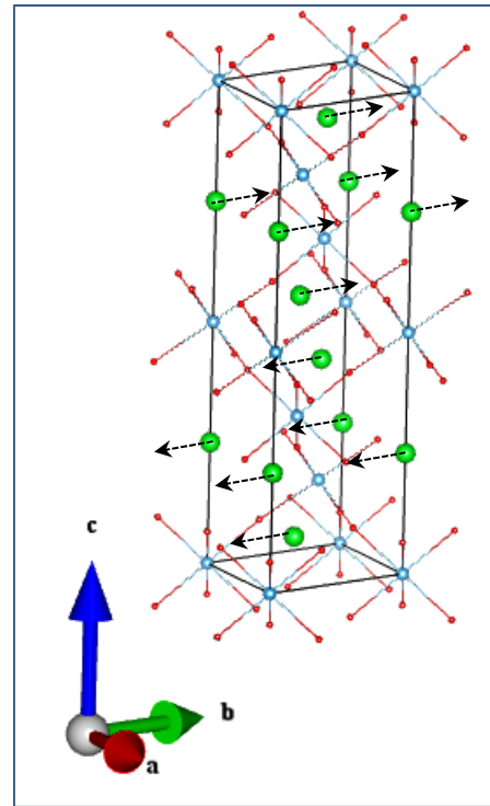
Sr_Eg (1_2)
