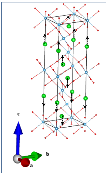
Sr_A2g
