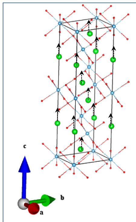
Sr_A2u
