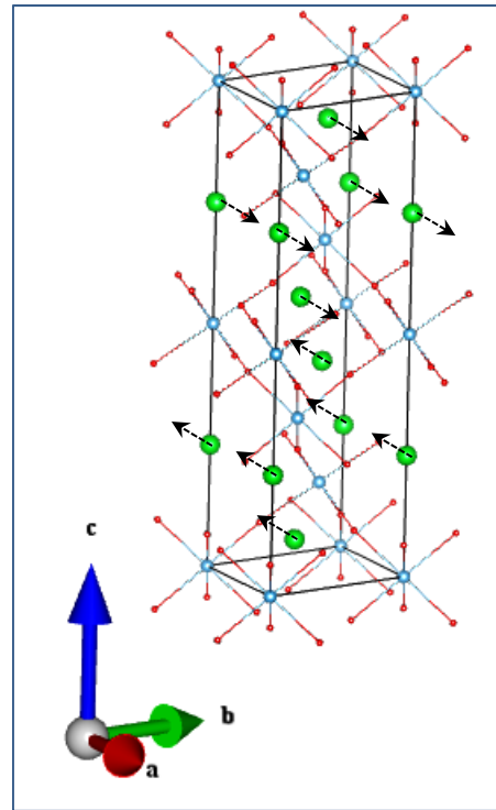
Sr_Eg (1_1)
