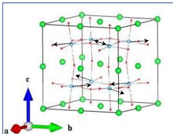
Ti_B 1u (1_1)
