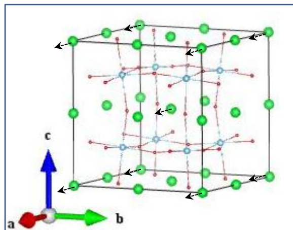
Sr 2 Eu (1_1)
