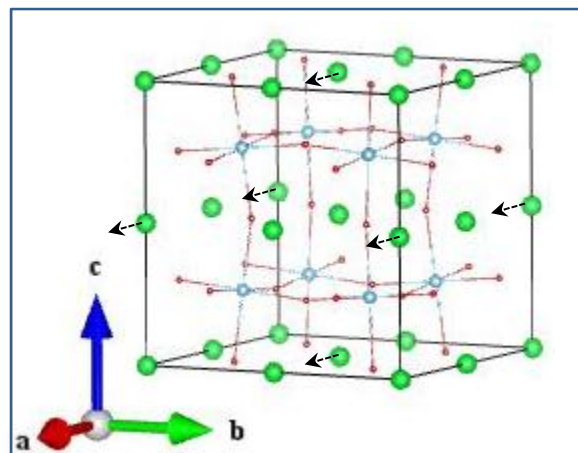
Sr 3 Eu (1_1)
