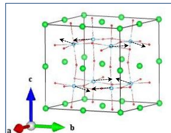
Ti_B 2u (1_1)
