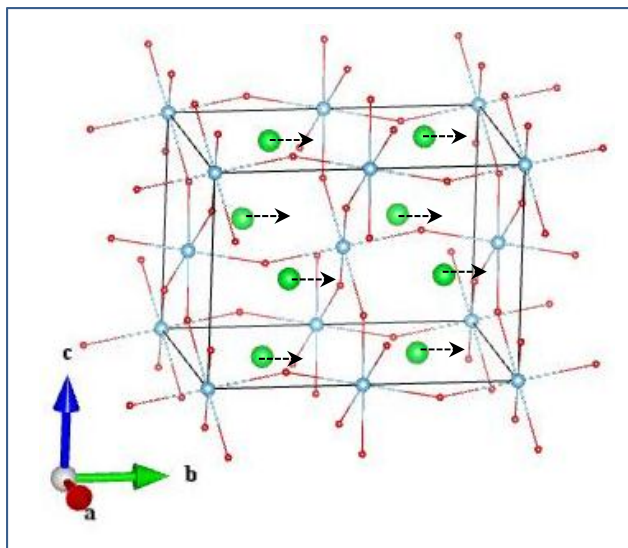
Sr_B 2u
