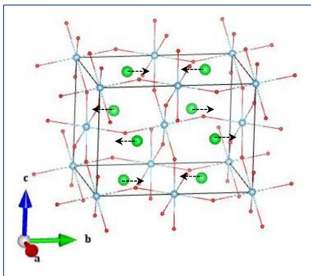
Sr_B 3g
