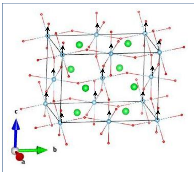
Ti_B 1u (1_1)
