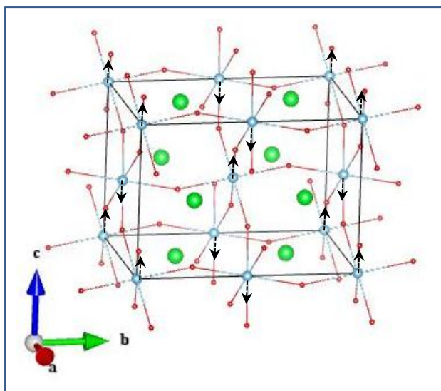
Ti_B 2u (1_1)
