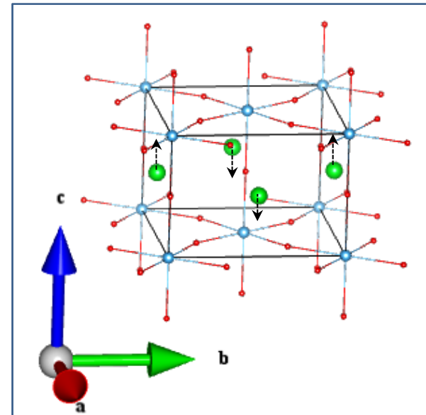
Sr_B 1u (1)
