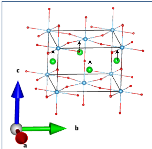
Sr_A 2u (1)
